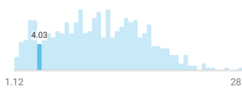
Forward passes / 90
